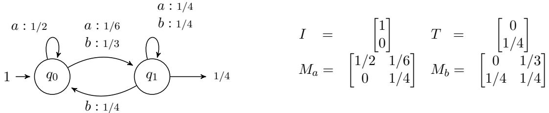
Figure 1: A weighted automaton and the equivalent linear representation.
